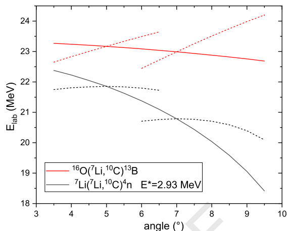
Fig. 3. Angle dependence of the two reactions {}^{16}\text{O}({}^7\text{Li}, {}^{10}\text{C}){}^{13}\text{B} and {}^7\text{Li}({}^7\text{Li}, {}^{10}\text{C}){}^4\text{n} for a total excitation energy of the {}^{10}\text{C} plus 4 neutron system of 2.93 MeV. In the dashed curves the kinematic correction (only linear term) for the {}^7\text{Li}+{}^7\text{Li} reaction and for the spectrograph at 7^\circ and at 5^\circ is taken into account. For the {}^{16}\text{O}({}^7\text{Li}, {}^{10}\text{C}){}^{13}\text{B} reaction the shift is then overcompensated.
